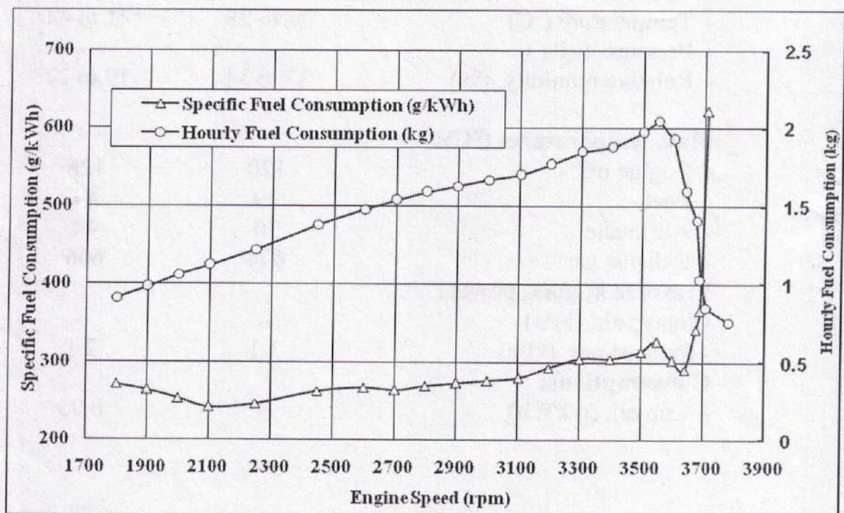
Fig. 4 ENGINE PERFORMANCE TEST (NATURAL AMBIENT)
