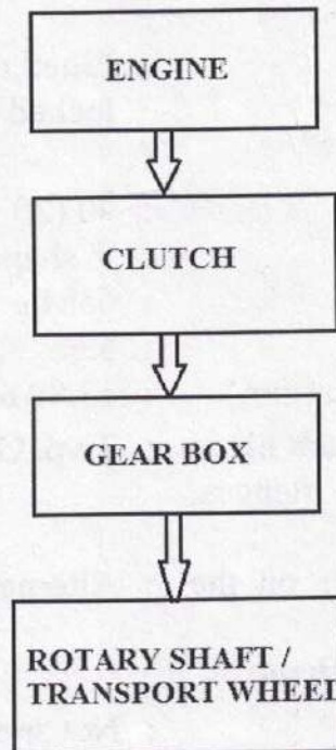
Fig. 2 Schematic power flow diagram
