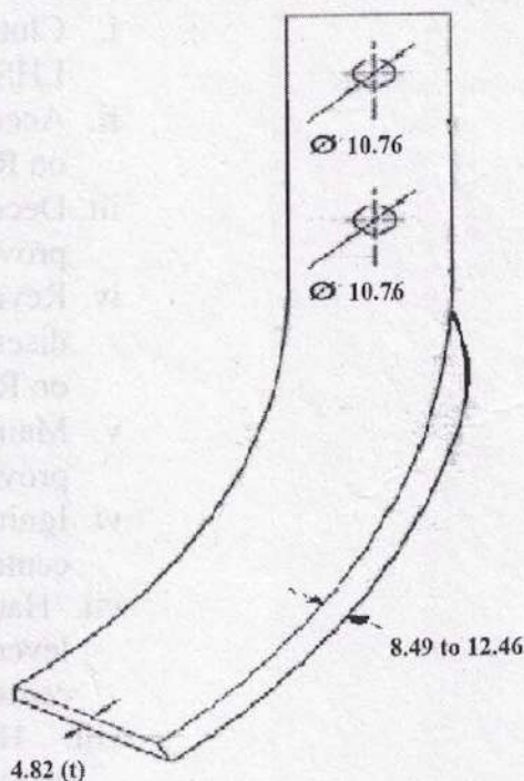
Fig. 3 Rotary blade (All dimensions in mm)
