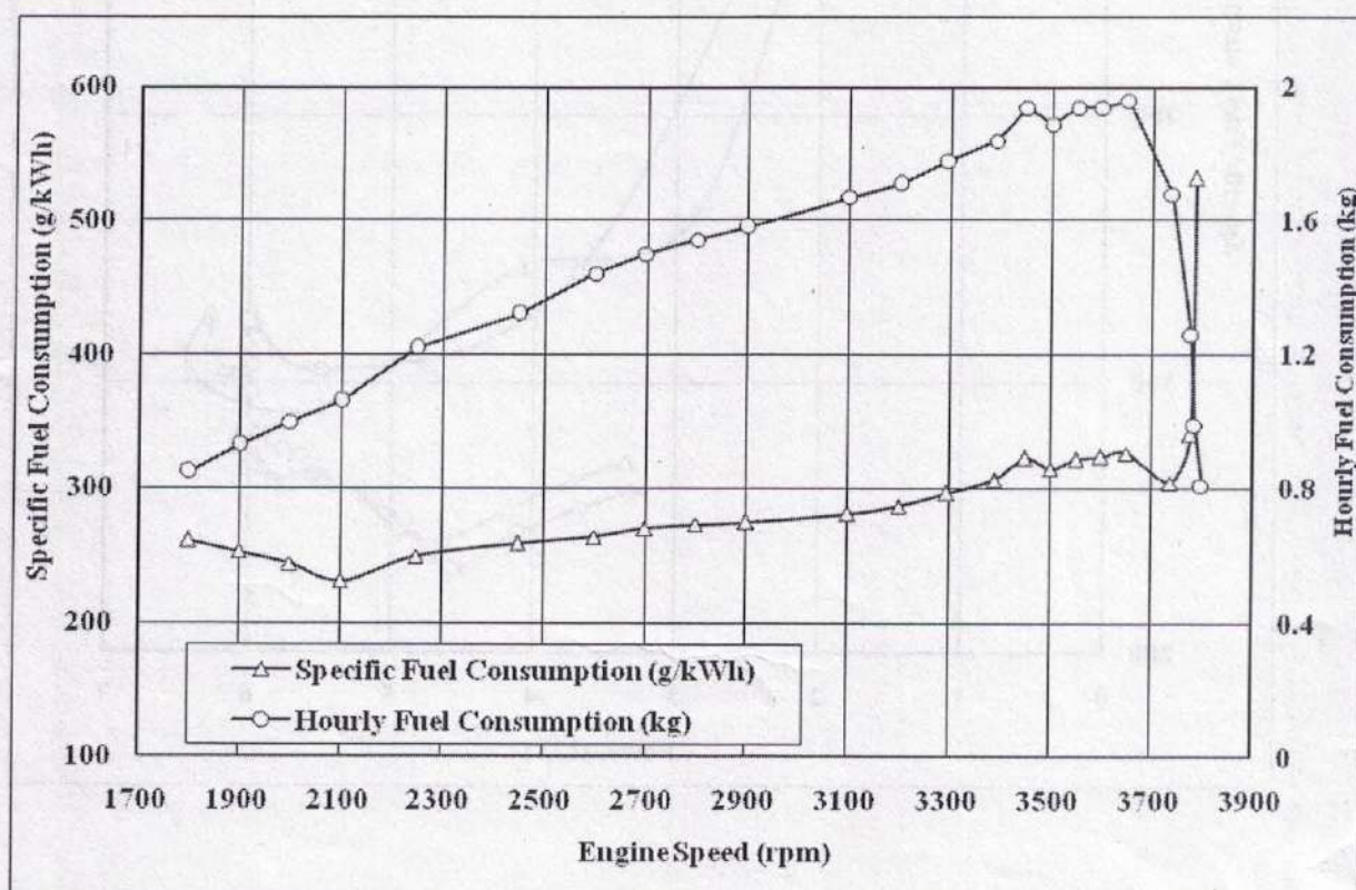
Fig. 5 ENGINE PERFORMANCE TEST (HIGH AMBIENT)
